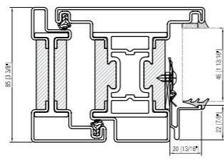
DOOR open out interior glazing bead
