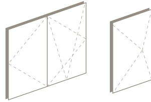
SINGLE CASEMENT up to: 5' x 10' FRENCH CASEMENT up to: 10' x 10' AWNING up to: 7' x 2' HOPPER up to: 7' x 2' PIVOT WINDOW up to: 6' x 7'3"
